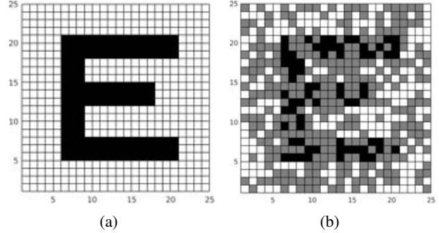
Figure 2: (a) Ground truth map of dimension 25 \times 25 used in the 2-D simulation. (b) 300 samples were taken randomly from the map in (a) without repetition.
